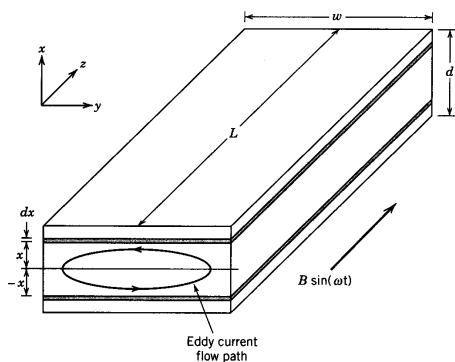
Figure 4: Eddy currents in the steel laminations of a transformer 3
